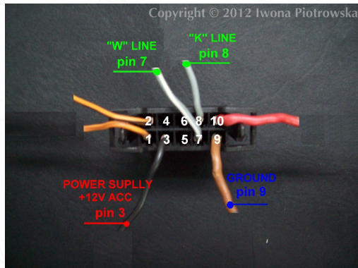
d) 10-pin immobiliser plug (e.g. certain VW T4 without CAN)
