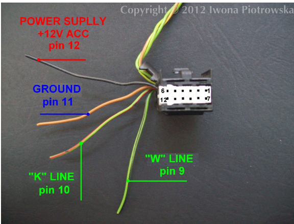
c) 12-pin immobiliser plug
